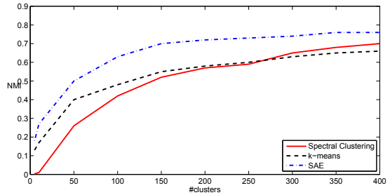
Figure 1: Clustering Results on DIP.
