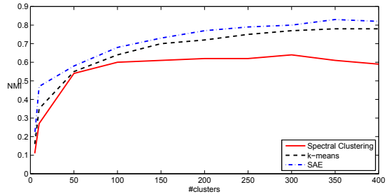
Figure 2: Clustering Results on BioGrid.
