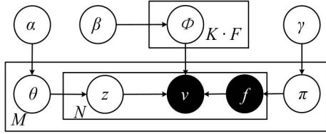
Fig. 6. Graphical model of LDAC, where M, N, F, K are the number of context profiles, contextual feature-value pairs, contextual features, and latent context topics, respectively; \alpha, \beta and \gamma are the prior parameters.
