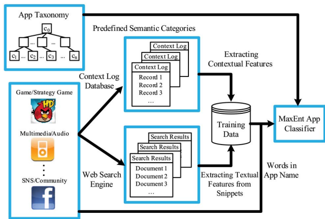
Fig. 4. Framework of our App classification approach.
