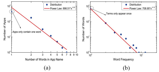
Fig. 7. Distribution of (a) number of mobile Apps with respect to the name length, and (b) number of unique words in App names with respect to their appearing frequency in our real-world data set.
