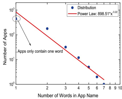
Fig. 1. Distribution of the number of mobile Apps with respect to the name length in our real-world data set.
