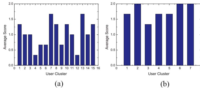
Fig. 13. Segmentation performance based on (a) original App vectors, and (b) App category vectors.
