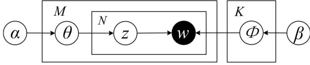
Fig. 5. Graphical model of LDA, where M , N , and K are the number of category profiles, words, and latent topics, respectively; \alpha and \beta are the prior parameters.
