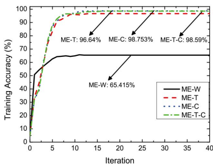
Fig. 11. Values of training accuracy per iteration of training ME-W, ME-T, ME-C and ME-T-C.
