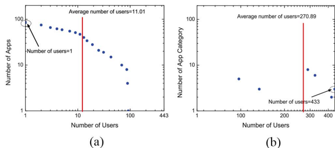
Fig. 12. Distributions of the number of used (a) Apps, and (b) categories with respect to the number of users.
