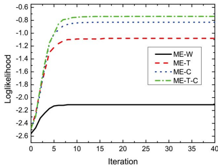
Fig. 10. Objective function values per iteration of training ME-W, ME-T, ME-C and ME-T-C.
