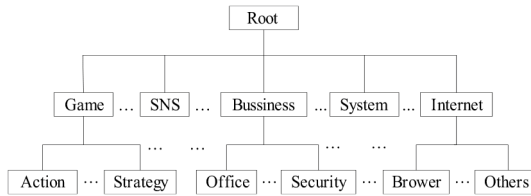
Fig. 2. Example of the mobile App taxonomy.
