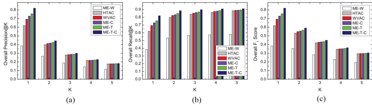
Fig. 9. Overall performance of each classification approach with different evaluation metrics in the cross validation. (a) Overall Precision@K. (b) Overall Recall@K. (c) Overall F1 Score.
