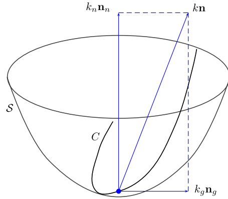
Fig. 3. The curvature vector k_n of curve C on \mathcal{S} has two orthogonal components: the normal curvature vector k_n n_n and the geodesic curvature vector k_g n_g .
