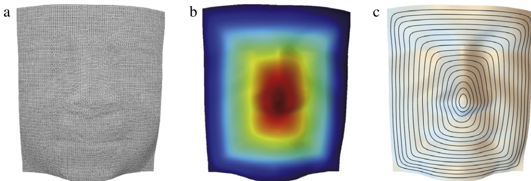
Fig. 9. Contour parallel tool path for the face model. (a) Meshing result; (b) optimal scalar function; (c) the generated tool path.
