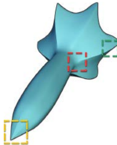
Constructed Manifold
