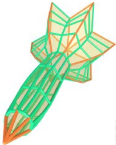
Domain
