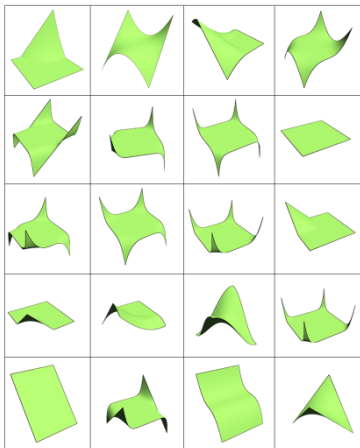
Dictionary
