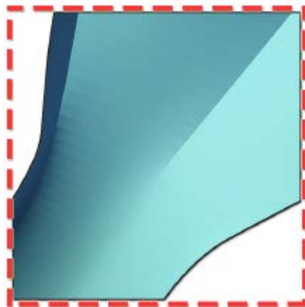
Dart
