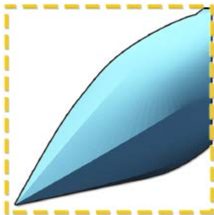
Cusp
