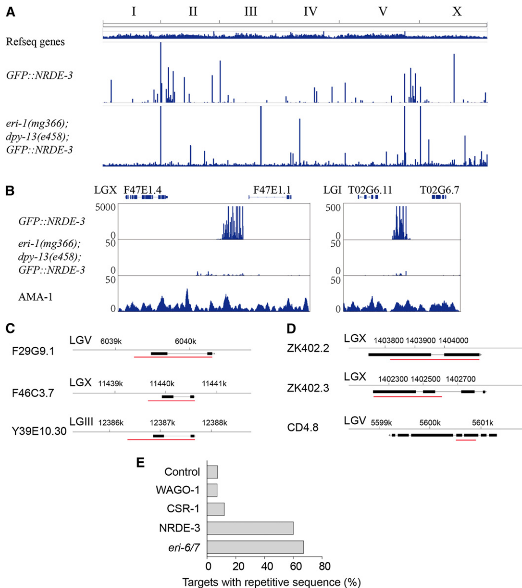
Figure 6 Nuclear RNAi targets distinct genomic loci. (A) NRDE-3-associated small RNAs were mapped to the C. elegans genome and displayed using the integrative genomics viewer (IGV). (B) NRDE-3-associated small RNAs target intergenic regions. The left panel indicates X-cluster siRNAs on chromosome X, which has the most NRDE-3-bound small RNA reads (Guang et al. 2008). AMA-1 (RNA polymerase II) ChIP-seq datasets were retrieved from GSM677643 of the modENCODE project to identify the binding region of AMA-1 in L4 wild-type animals (Gerstein et al. 2010). (C and D) The genes targeted by NRDE-3-associated siRNAs were blasted against the genome. Shown are examples of the gene groups that share high sequence similarity with a cutoff of >90% nt identity over a stretch of >200 nt of sequence. The red bars indicate the regions with sequence homology. (E) The repetitiveness of the targets of three secondary Argonaute proteins, including WAGO-1, CSR-1, and NRDE-3, and the targets of eri-6/7 were compared by using a criteria of >90% nt identity in a stretch of >200 nt sequence to one or more of the other targeted genes or genomic loci. A set of randomly selected genes ( n = 40 ) was used as a control.
