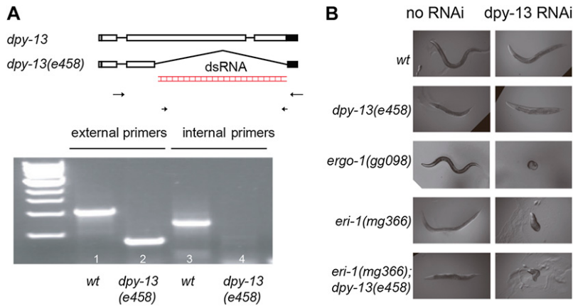
Figure 1 Off-target silencing occurs in enhanced RNAi animals. (A) Gene structure of dpy-13 . Recessive dpy-13(e458) is a 723-bp deletion, which removed 71% of the protein coding region and the translation stop codon. All of the conserved Gly-X-Y repeats, which are essential for the function of collagens, are deleted. wt, wild-type. (B) Feeding RNAi targeting the dpy-13(e458) -deleted sequence induced a worm-ball-like superdumpy phenotype in eri animals. L1 animals were fed dpy-13 dsRNA.
