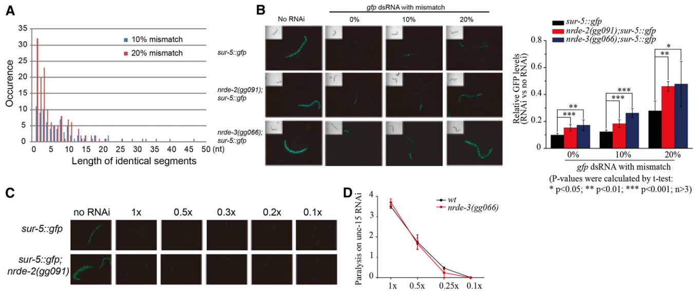
Figure 4 Nuclear RNAi is required for gfp dsRNA-induced off-target silencing. (A) Sequence comparison of mutagenized gfp dsRNAs that were generated by error-prone PCR. At the 20% mismatch level, one 21-nt segment is identical in sequence to wild-type GFP. (B) Left: L1 animals expressing sur-5::gfp were fed gfp dsRNAs with 0, 10, or 20% sequence mismatch. Right: GFP levels were quantified by ImageJ and normalized to control animals. (C) L1 animals expressing sur-5::gfp were fed a diluted series of gfp dsRNA. The dilution series was performed by mixing overnight cultures of bacteria expressing dsRNA with HT115 control bacteria. (D) L1 animals were fed a diluted series of unc-15 dsRNA, and their phenotypes were scored 3 days later.
