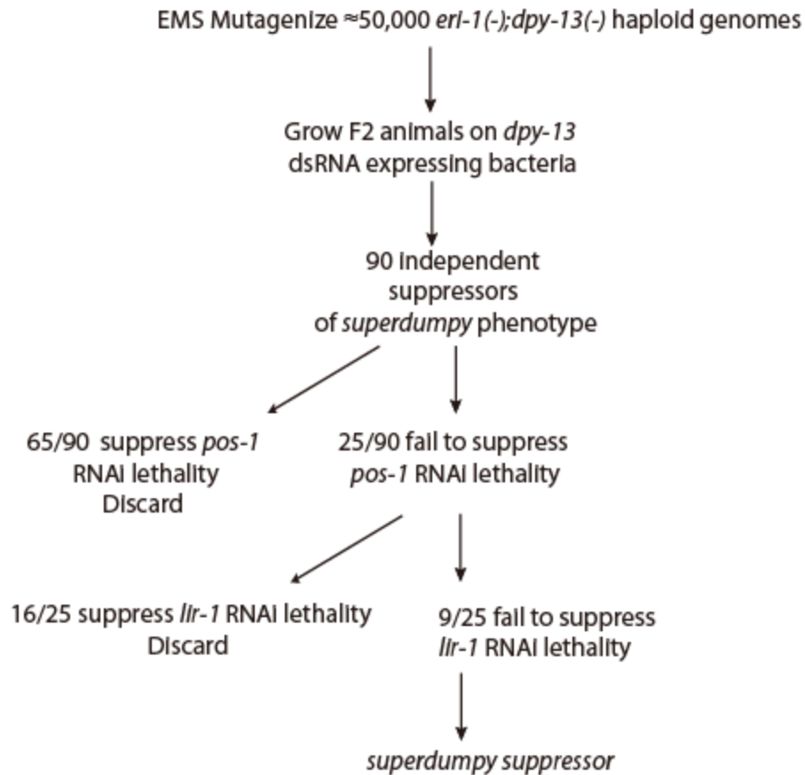
Figure S2 Schematic diagram of genetic screening to search for factors required for off-target silencing. eri-1(mg366); dpy-13(e458) animals were chemically mutagenized and searched for mutants that suppressed RNAi off-target effect but were dispensable for pos-1 and lir-1 RNAi. pos-1 RNAi leads to unhatched F1 embryos; animals that are resistant to pos-1 RNAi likely carry mutations in the core components of RNAi machinery. lir-1/lin-26 genes are expressed in an operon; they are co-transcribed as a polycistronic pre-mRNA, which is spliced into distinct mRNAs in the nucleus before export to the cytoplasm. lir-1(-) mutant animals are viable. Loss of function alleles of lin-26 are inviable. RNAi targeting lir-1 induces a lethal phenotype by silencing the nuclear-localized lir-1/lin-26 RNA. nrde mutant animals are viable following lir-1 RNAi, because nrde genes are required to silence the nuclear-localized lir-1/lin-26 RNA (Guang, 2008). Similarly, nrde genes are required to silence the nuclear-localized lin-15b/lin-15a polycistronic RNA. Nine mutants that were specifically defective in off-target silencing were isolated. Mutants were mapped by snp-SNP mapping and candidate genes are sequenced.
