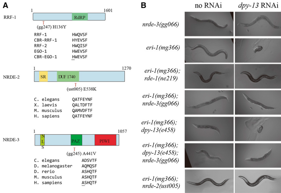
Figure 2 (A) Genetic screening identified the alleles of rrf-1 , nrde-2 , and nrde-3 that are required for off-target gene silencing. eri-1(mg366); dpy-13(e458) animals were chemically mutagenized and screened for mutants that suppress off-target RNAi effect but are still sensitive to pos-1 and lir-1 RNAi. The mutants were mapped via the snp-SNP technique and sequenced. Underlining indicates the mutated amino acids. RRF-1, RRF-2, and EGO-1 are RNA-dependent RNA polymerases. CBR-EGO-1 and CBR-RRF-1 are C. briggsae genes. (B) Nuclear RNAi is required for dpy-13 dsRNA-induced off-target silencing. L1 animals of the indicated genotypes were fed dpy-13 dsRNA, and images were obtained 3 days later. RDE-1 is a primary Argonaute protein that is a prerequisite for feeding RNAi (Steiner et al. 2009). dpy-13 RNAi failed to produce any visible silencing effects in eri-1(mg366); rde-1(ne219) animals.
