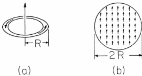
Figure 9.01 (a) Current i in loop of radius R gives dipole moment \mathbf{m} . (b) Spherical material of radius R has dipole moment approximated as the sum of atomic dipole moments.
