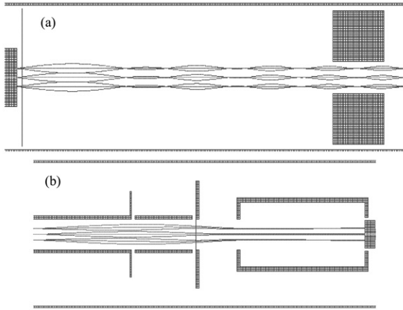
Fig. 2. The processes of positron transportation (a) and focusing on the target (b).
