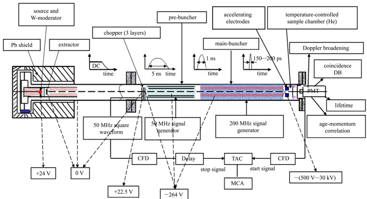
Fig. 1. Schematic diagram of a slow pulsed positron beam.
