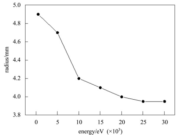
Fig. 3. The variation in focusing radius with accelerated energies.
