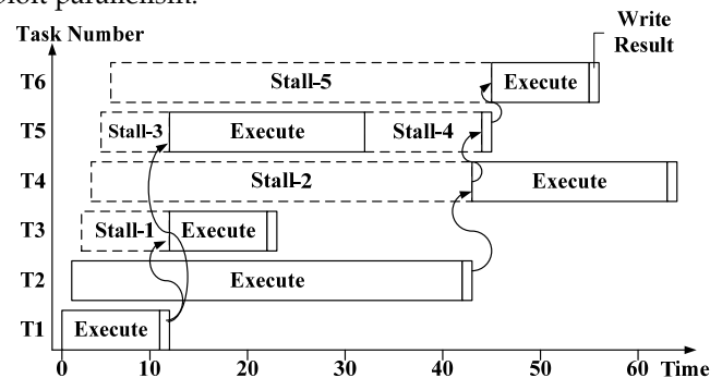
Fig. 12 Timing Diagram of the sample task sequence in Table 3
