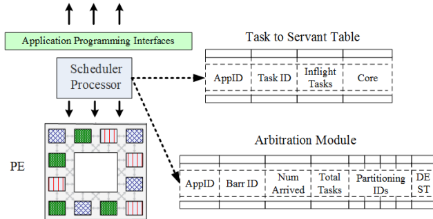
Fig. 4 Task to Servant Table and Arbitration Module.
