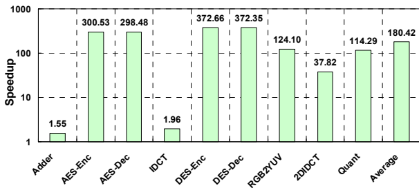
Fig. 8. Performance improvement due to service substitution.
