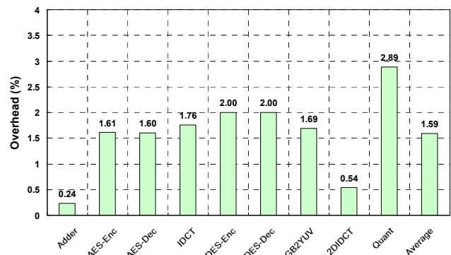
Fig. 7. Overhead of componentization over the original version.
