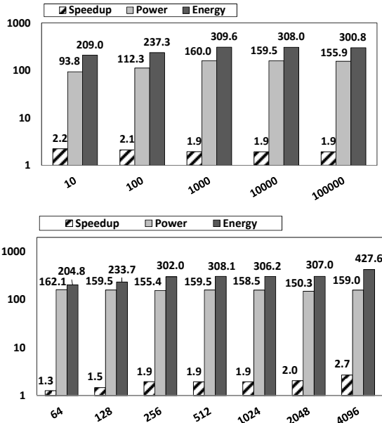
Fig. 13. Experimental results of hardware arbitration with different data sizes and task scales
