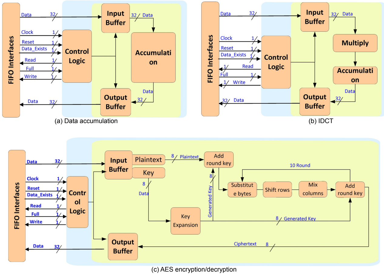
Fig. 6 Data accumulation, IDCT, and AES hardware servants.
