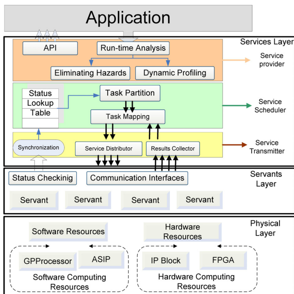
Fig. 3 Hierarchical level model of SoSoC is comprising three layers.
