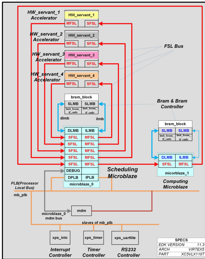
Fig. 5. SoSoC Prototype in FPGA.
