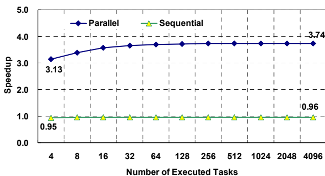
Fig. 9. Peak speedup against execution in a single core.
