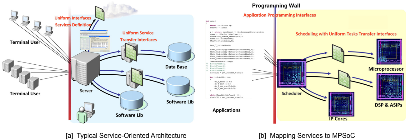
Fig. 1 Typical SOA concepts and the corresponding services in MPSoC.
