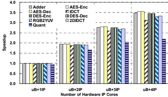
Fig. 11. Speedup with different number of hardware IP Cores
