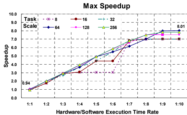
Fig. 10. The impact of Different Hardware Execution Time.
