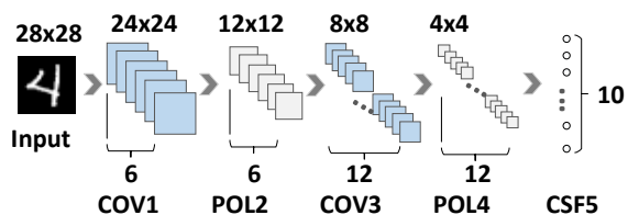
Fig. 14. Neural network hierarchy is containing different layers.
