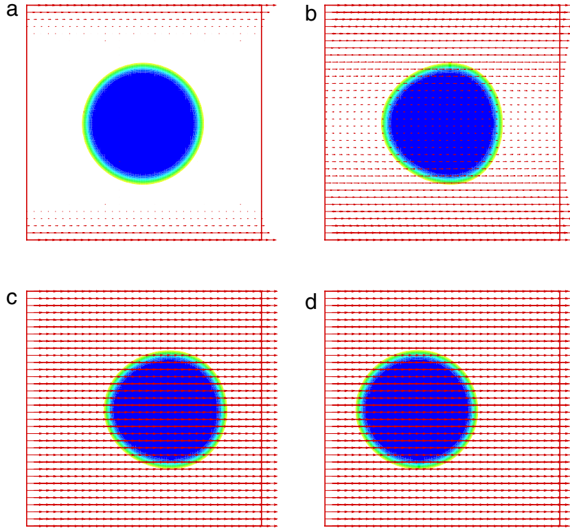
Fig. 1. Velocity vectors and density contours of a moving bubble. The computational domain is 100 \times 100 \text{ lu}^2 . The relaxation parameters for the blue (gray) and white phases are \tau_1 = 0.6 and \tau_2 = 1.0 , respectively. (a) tu_w/L = 0.005 ; (b) tu_w/L = 0.2 ; (c) tu_w/L = 2.8 ; (d) tu_w/L = 3.6 . (For interpretation of the references to colour in this figure legend, the reader is referred to the web version of this article.)
