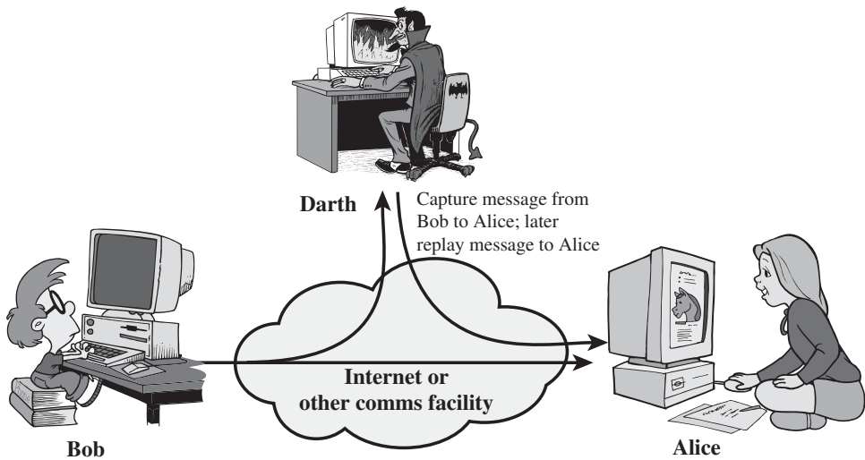
(b) Replay
