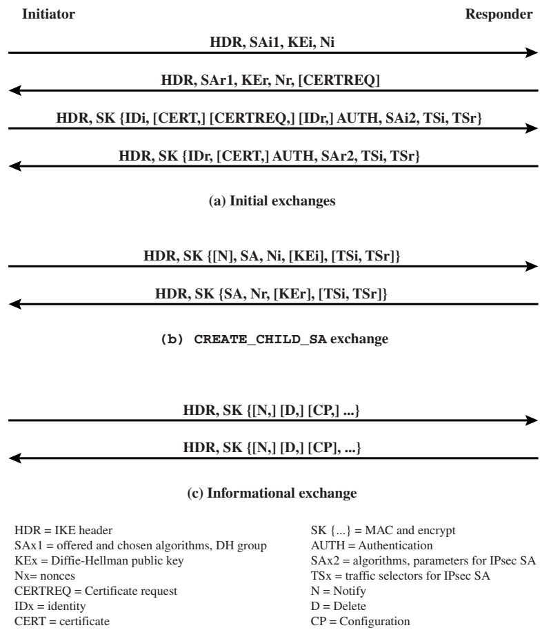
Figure 19.11 IKEv2 Exchanges
