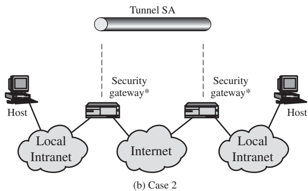
Figure 19.10 Basic Combinations of Security Associations
