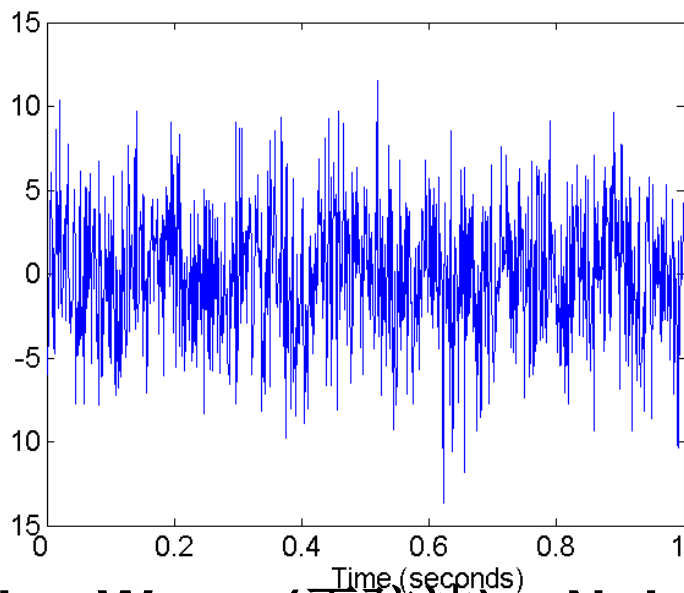
Two Sine Waves(正弦波) + Noise
