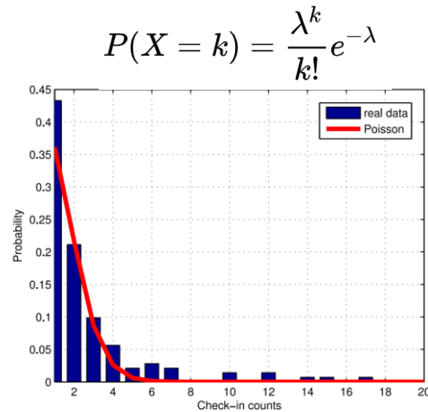
Fig. 3. The check-in counts distribution of a randomly selected user and a Poisson approximation of this distribution (Foursquare dataset).
