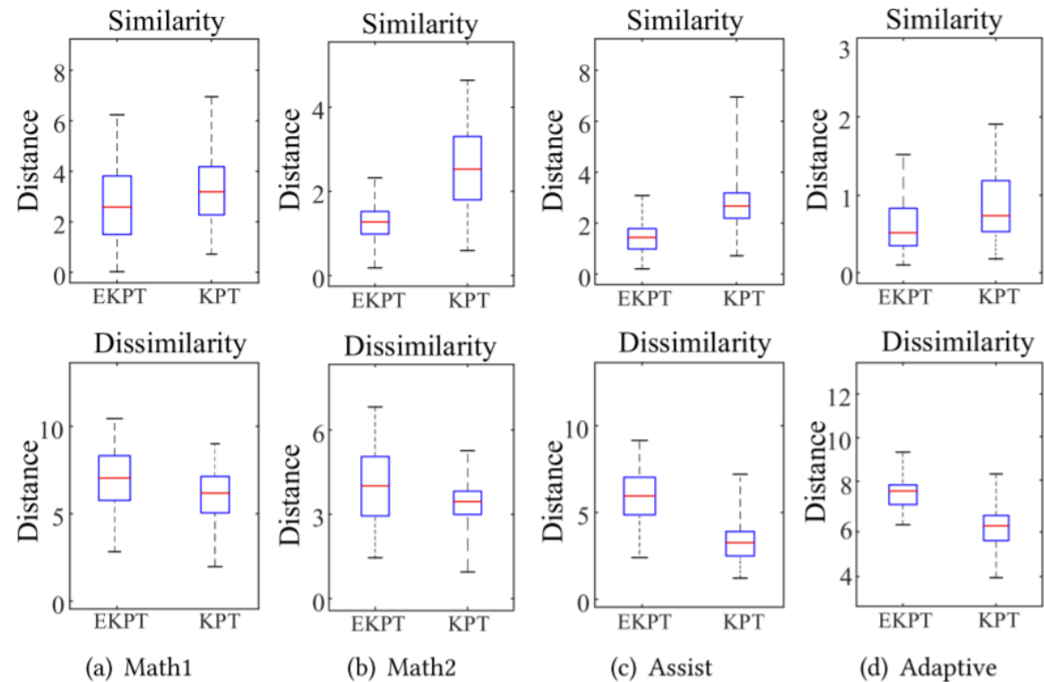
Fig. 11. Results comparison of exercise relationship with EKPT and KPT in all datasets.
