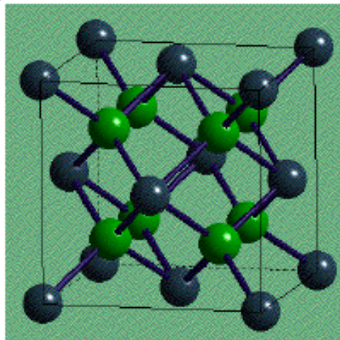
Fluorite A-cell
