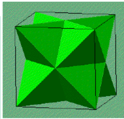
\text{FCa}_4 Tetrahedra
