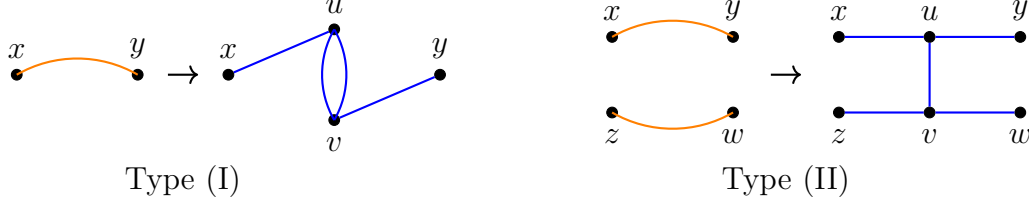
Figure 2: The operation G \leftrightarrow G'
