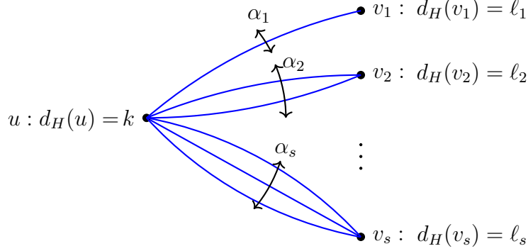
Figure 1: The multi-star S_{(k; \ell_1, \dots, \ell_s; \alpha_1, \dots, \alpha_s)}(H)
