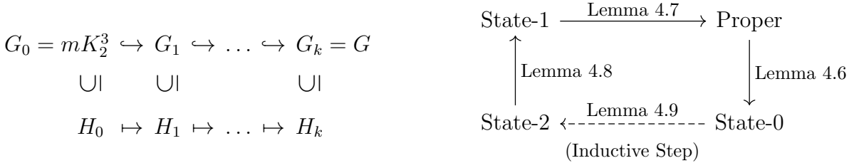
Figure 3: The overall proof of Theorem 1.3
