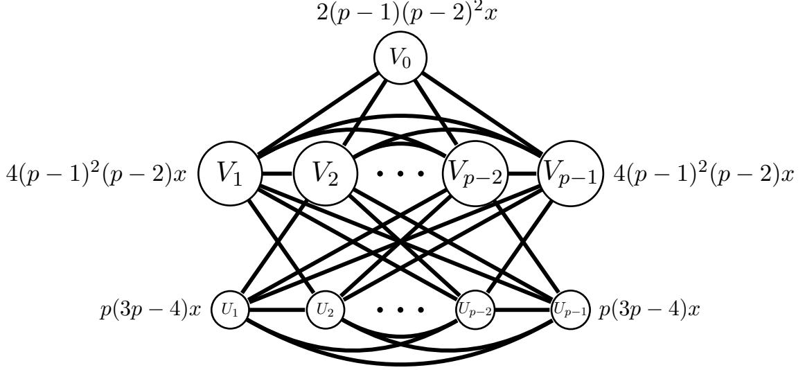
Figure 1. Constructions for the upper bounds of Theorem 1.2 and 1.3.
