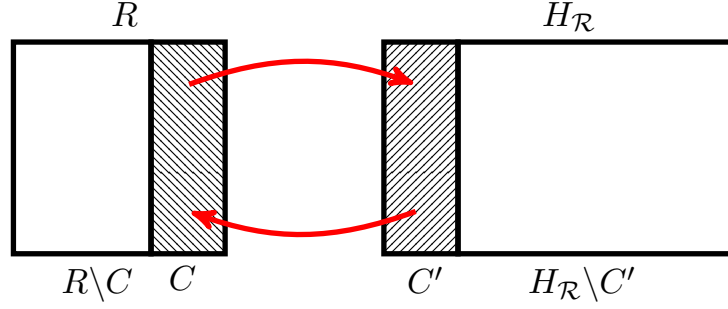
Figure 2. The proof of Lemma 4.1
