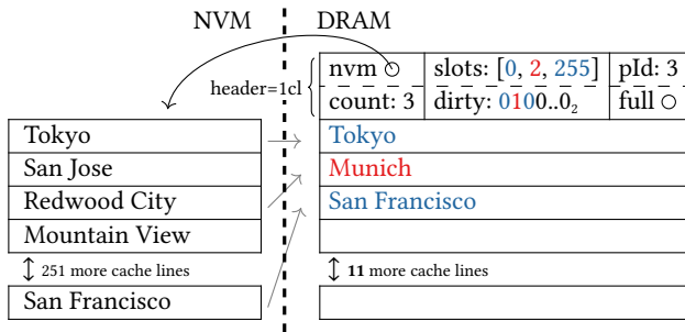
Figure 4: Mini Pages – The slots array indicates which cache lines are loaded (max 16). If promoted, full1 points to the full page.
