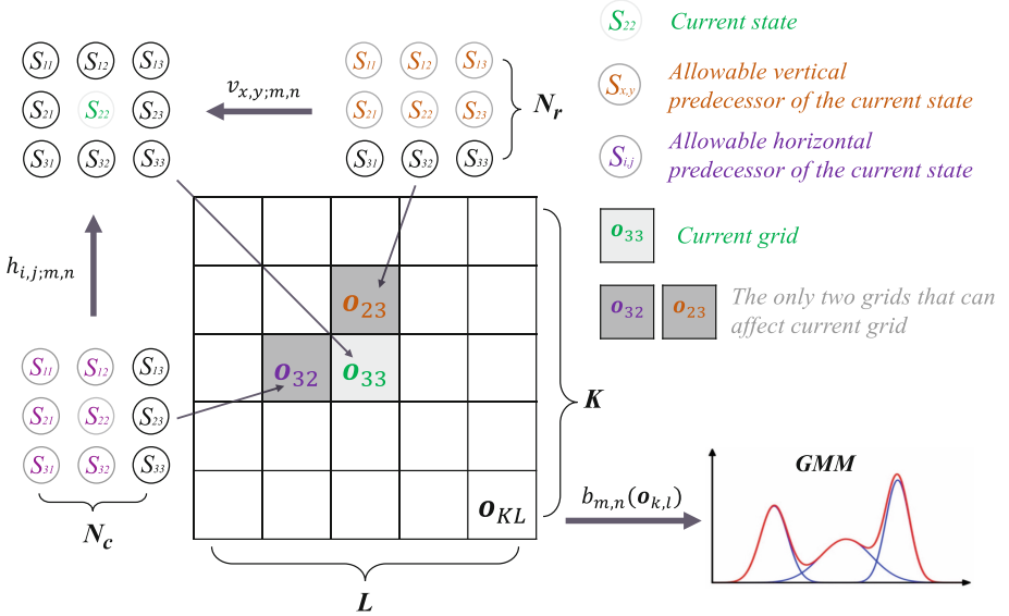
Fig. 1. 2D-GMM-HMM system.
