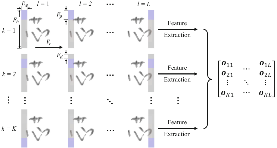
Fig. 2. Feature extraction method in 2D-HMM.
