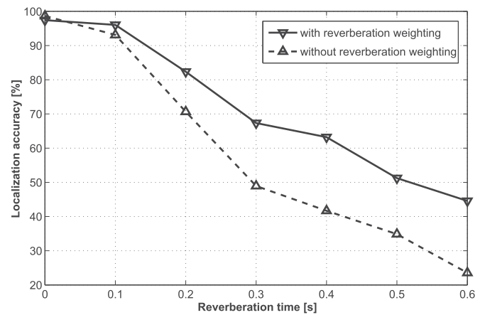
Fig. 8. Comparison of localization accuracies between the method with and without reverberation weighting where tolerance = 0°.
