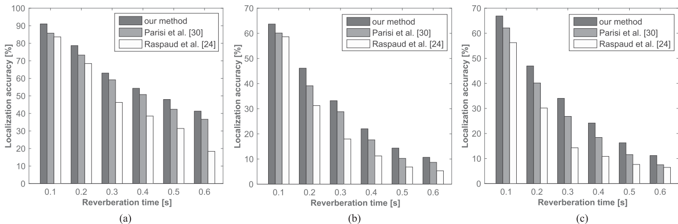
Fig. 10. Localization accuracies of different azimuths \theta = (a) -15^\circ ; (b) -80^\circ ; (c) 80^\circ at different reverberation times where tolerance = 0^\circ .
