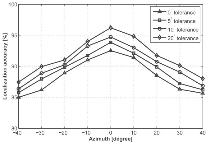
Fig. 14. The average localization accuracies of our method for different tolerances and directions in realistic environments.
