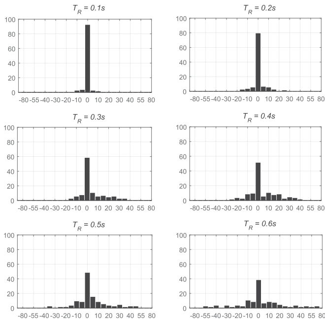
Fig. 9. Histograms of the localization results where azimuth \theta = 0^\circ and reverberation time ranges from T_R = 0.1 s to T_R = 0.6 s.
