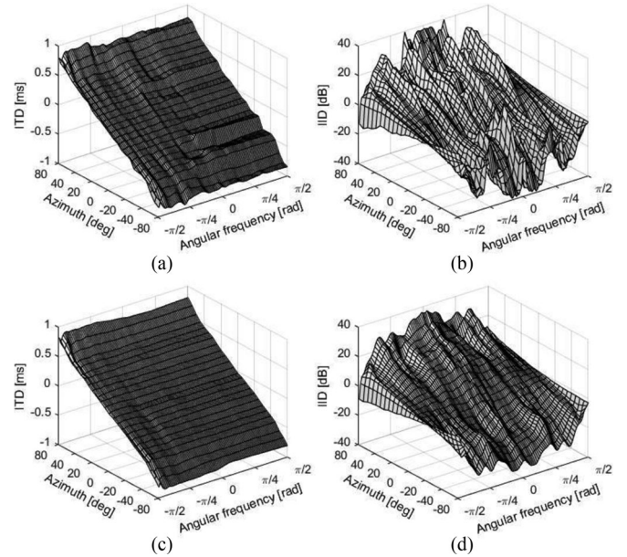
Fig. 3. Binaural cues distribution versus azimuth and angular frequency in the CIPIC HRTF database. (a) ITD and (b) IID for subject #21. (c) Averaged ITD and (d) averaged IID over all subjects.
