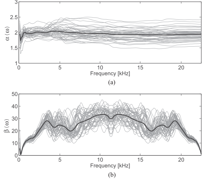
Fig. 4. The changing trends of the scaling factors for ITD (a) and IID (b) model in terms of frequency and subject.
