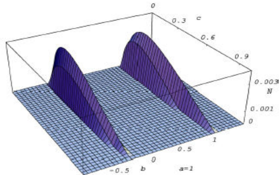
FIG. 2. Depiction of N = \max\{|\widetilde{\rho}_{AB}^{T(c_A, r_B)}| - h_a h_b, 0\} for a Horodecki 3 \times 3 bound entangled state as a function of b and c when a=0 (the top figure) and a=1 (the bottom figure), respectively.
