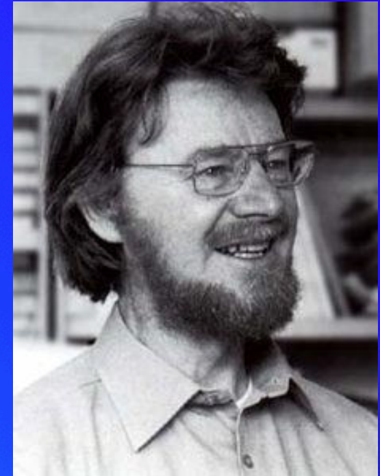
John Bell (1928-1990)
