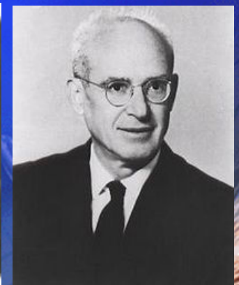
Nathan Rosen
