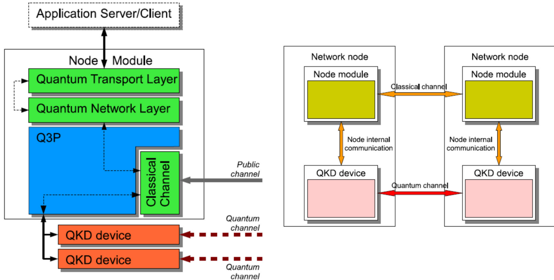
Figure 18. Design of the node module.
