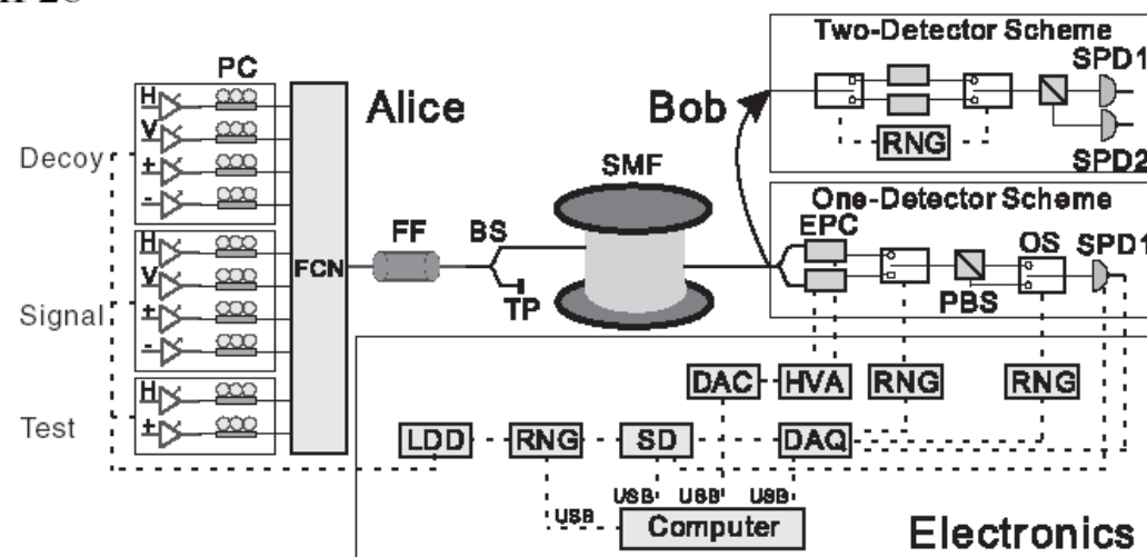
FIG. 1. Schematic diagram of the experimental setup. Solid lines and dashed lines represent the optical fiber and electric cable, respectively. See the text for the abbreviations.
