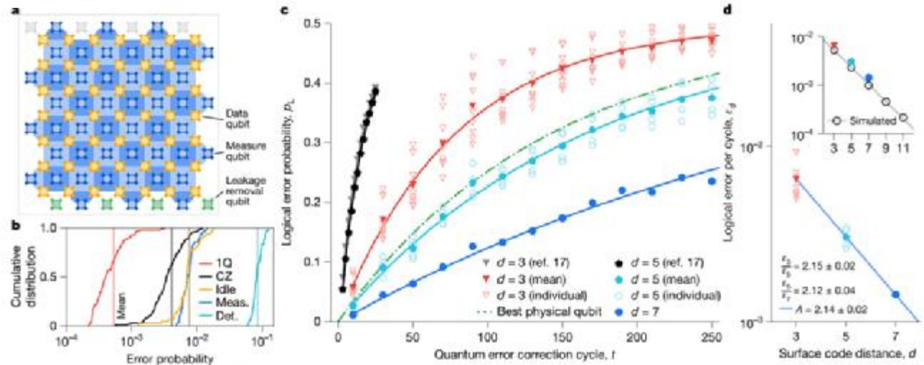
Fig. 1 | Surface code performance. a, Schematic of a distance-7 ( d=7 ) surface code on a 105-qubit processor. Each measure qubit (blue) is associated with a stabilizer (blue-coloured tile). Data qubits (gold) form a d \times d array. We remove leakage from each data qubit using a neighbouring qubit below it, with additional leakage removal qubits at the boundary (green). b, Cumulative distributions of error probabilities measured on the 105-qubit processor. Red, Pauli errors for single-qubit gates; black, Pauli errors for CZ gates; gold, Pauli errors for data qubit idle during measurement and reset; blue, identification error for measurement; teal, weight-4 detection probabilities (distance 7, averaged for 250 cycles). c, Logical error probability p_L for a range of memory experiment durations. Each data point represents 10^5 repetitions decoded with the neural
