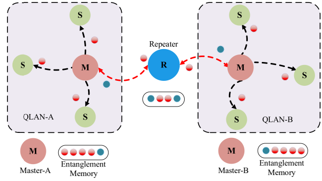
Figure 5. The establishment of slave-to-slave entanglement. Slave nodes in the same QLAN are entangled in pairs. And slave nodes in different QLANs establish entanglement by performing entanglement swapping on a quantum repeater chain.
