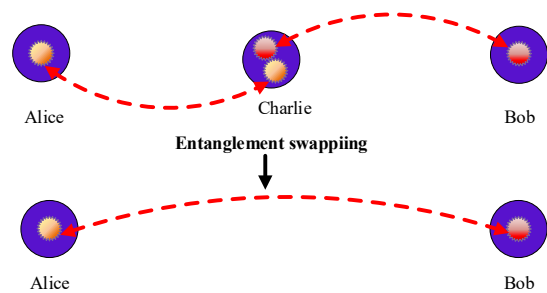
Figure 2. Entanglement swapping. Two short-distance entanglements can be extended to a remote entanglement between Alice and Bob by performing the LOCC operation on two un-entangled states that Charlie stores.
