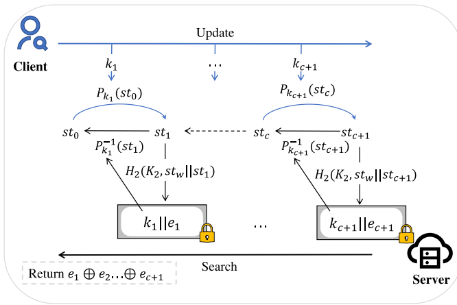
Fig. 6. An Extension of Our Scheme to Support Dynamic Updates
