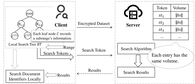
Fig. 5. Overview of Our Proposed Scheme
