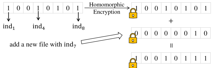
Fig. 3. An Example of the Bitmap Index
