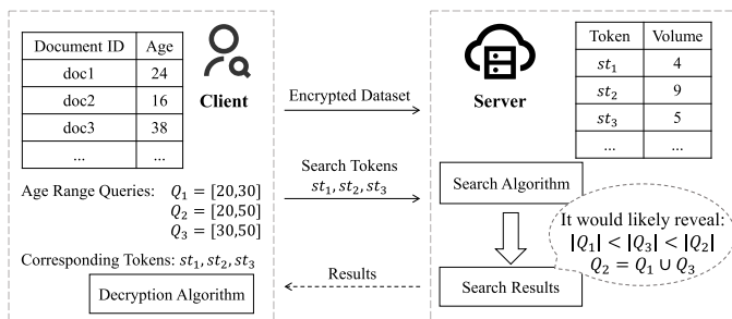
Fig. 1. An Example of Volume Leakage in Range SSE
