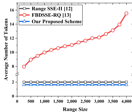
Fig. 8. Number of Tokens for Different Range Sizes
