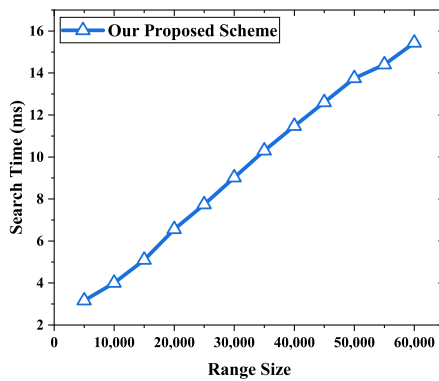
Fig. 10. Search Time of Our Proposed Scheme on Large-Scale Dataset
