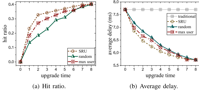
Fig. 5. Comparison of different router upgrading algorithms in different performance metrics at different upgrades.
