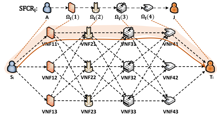
Fig. 3. Solving DRP-SFC on LFG
