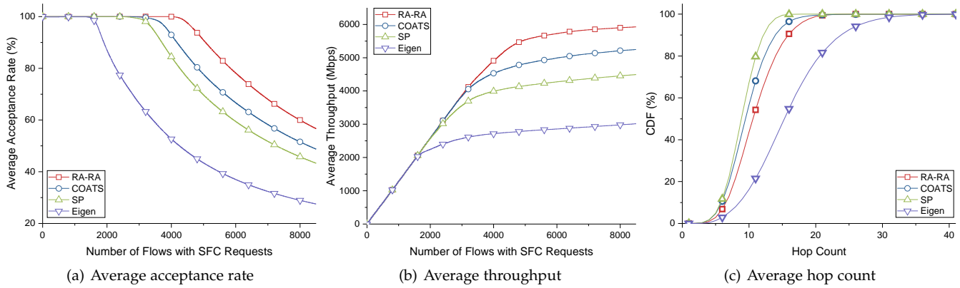
Fig. 5. The comparison of average acceptance rate, throughput and hop count
