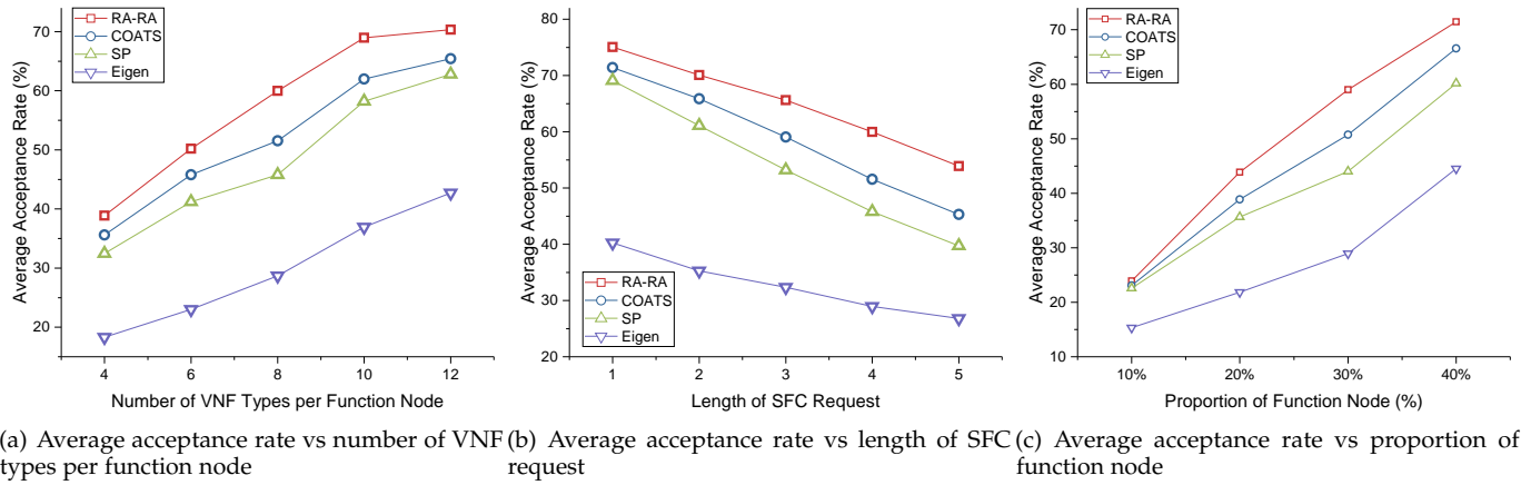
Fig. 7. Comparison of average acceptance rate in different scenarios
