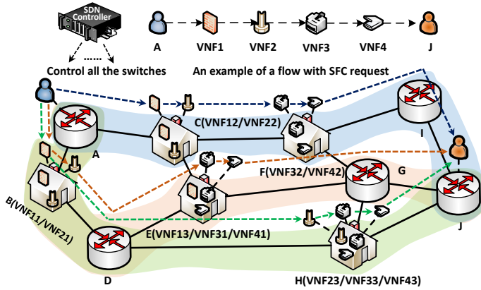
Fig. 1. VNF instance selection and path construction for flows with SFC requests in SDN and NFV-enabled network
