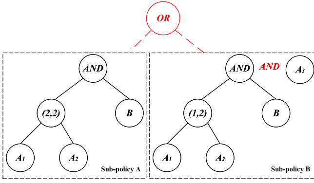
Fig. 5. Two sub-policies by the trivial solution.
