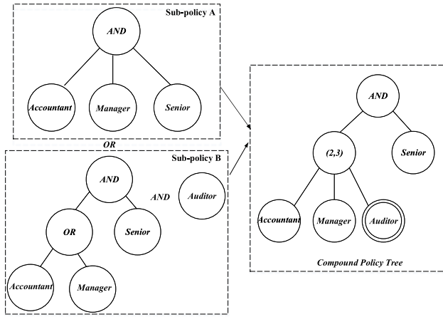
Fig. 1. An example of an access policy.
