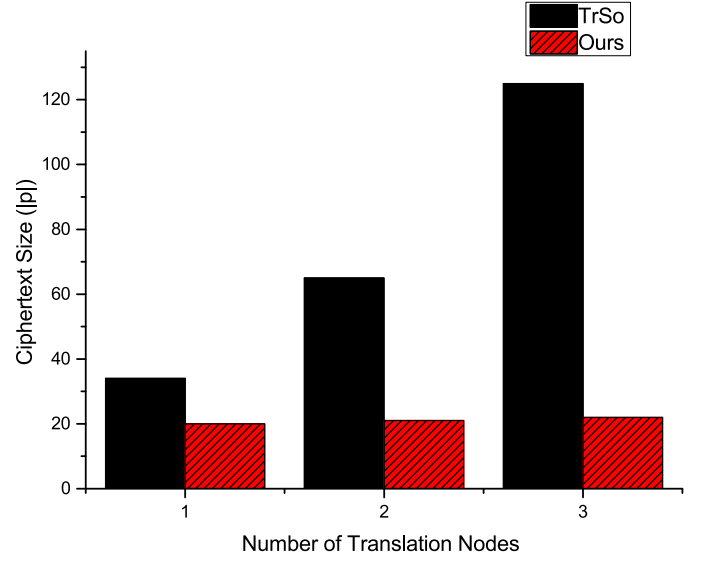
Fig. 9. Ciphertext size.
