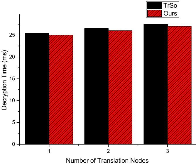
Fig. 8. Decryption time.
