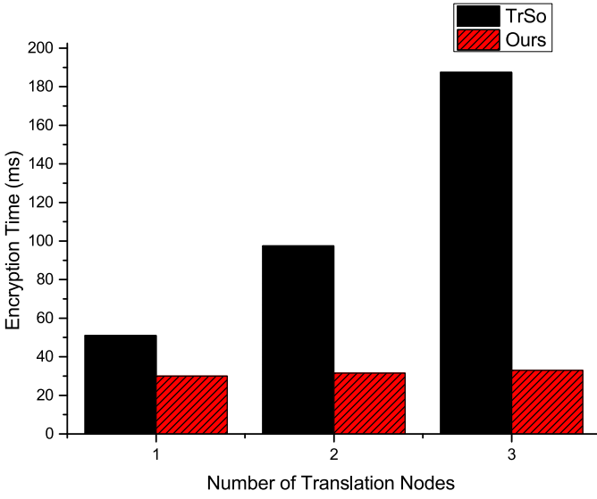
Fig. 7. Encryption time.
