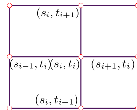
Fig. 8. A new basis vertex and its neighboring cells.
