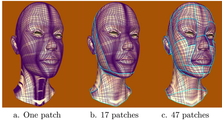
Fig. 15. Conversion of PHT-spline surfaces to TP-spline surfaces.
