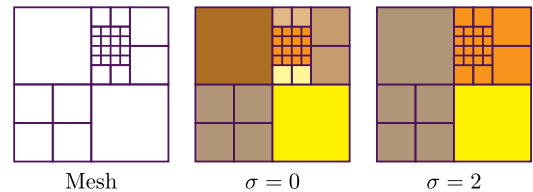
Fig. 14. Examples of hierarchical T-mesh segmentation.
