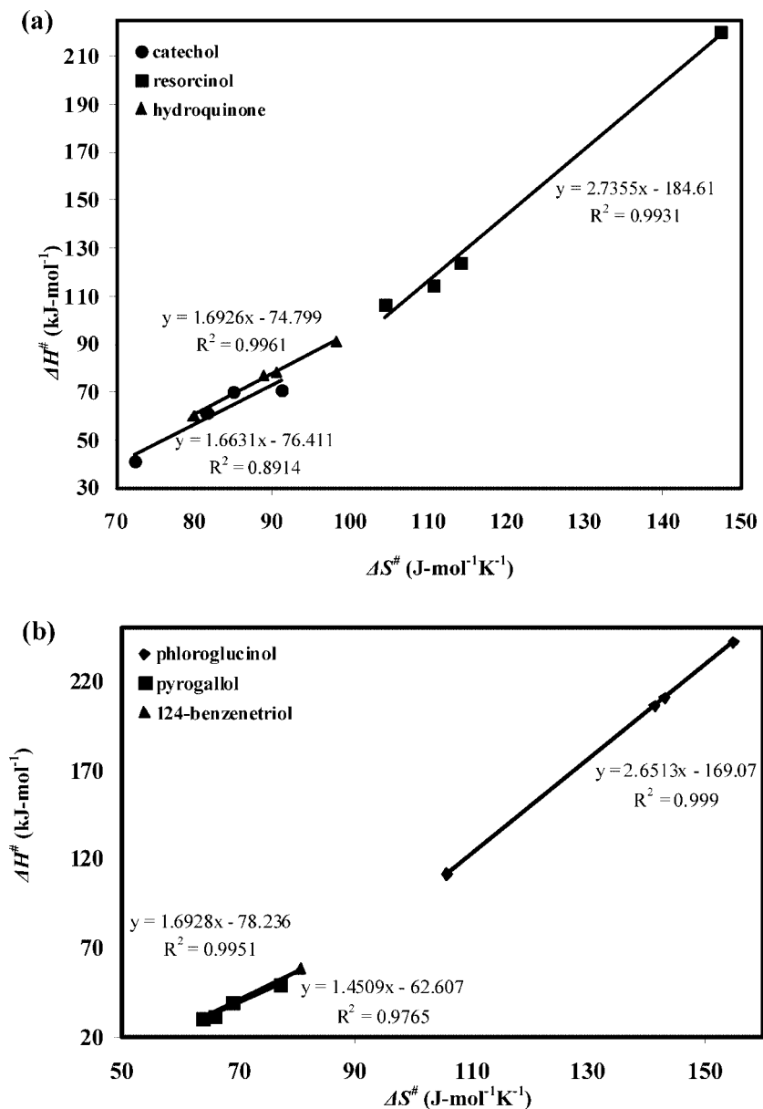
Figure 5. Activation enthalpy and entropy compensation for phenolics with (a) two OH groups and (b) three OH groups.
