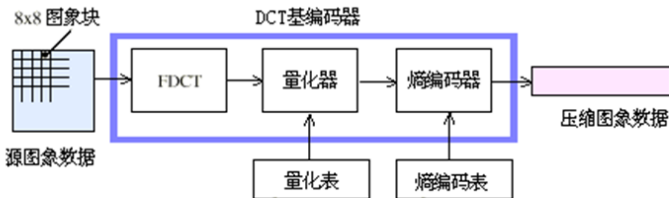
(a) DCT基压缩编码步骤
