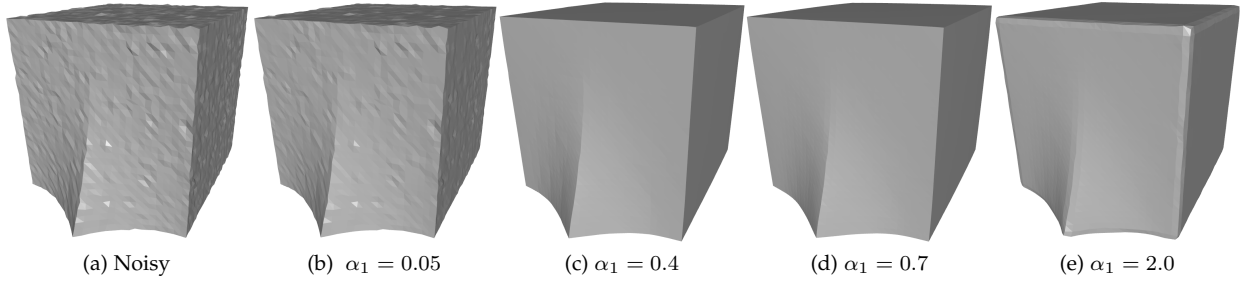
Fig. 6: Denoising results for varying \alpha_1 with fixed \alpha_0 and \beta . From left to right: noisy mesh (corrupted with \sigma = 0.1\bar{l}_e ), and results with increasing \alpha_1 .
