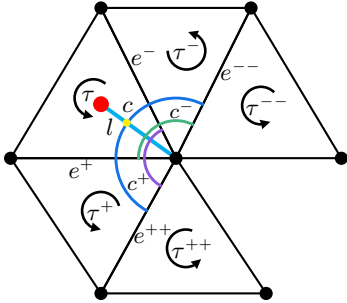
Fig. 3: Illustration of the definition of 2-form operator \bar{\mathcal{D}}_{\mathcal{E}} v . [[v]] is the 2-form jump over curve c plotted in blue, which passes through four edges ( e^{--}, e^-, e^+, e^{++} ) and attaches itself to line l . Auxiliary curve c^- passing through ( e^{--}, e^+ ) is plotted in green, and curve c^+ passing through ( e^-, e^{++} ) is plotted in purple.
