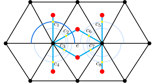
Fig. 4: Illustration of the definition of adjoint operator \tilde{\mathcal{D}}_{\mathcal{E}}^* \tilde{w} . B_2(e) is the set of curves associated with edge e , which refers to eight curves. The attached lines of curves in B_2(e) are also shown.
