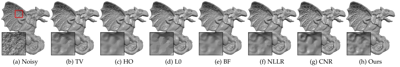
Fig. 12: Comparison of denoising results for Gargoyle, corrupted with \sigma = 0.25\bar{l}_e .
