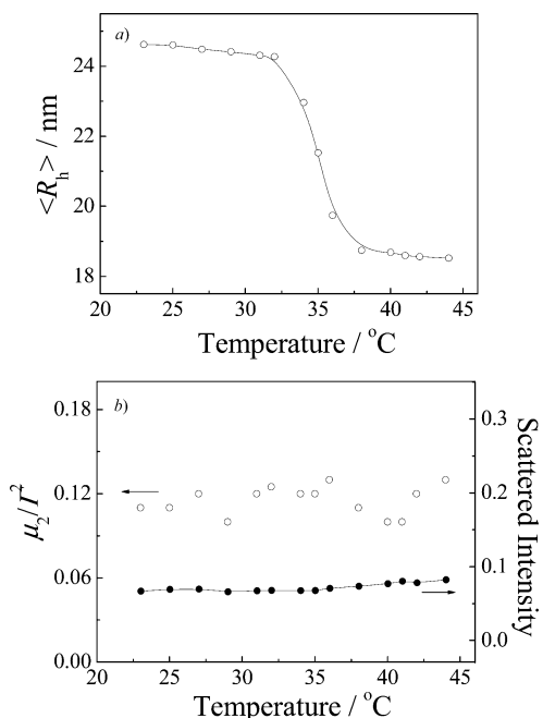
Figure 7. Variation of (a) intensity-average hydrodynamic radius, \langle R_h \rangle , and (b) scattered light intensity and polydispersity index ( \mu_2/\bar{I}^2 ) as a function of temperature at pH 9.0 obtained for a 0.01 g/L aqueous solution of SCL micelles of the PDEA- b -PDMA- b -PNIPAM triblock copolymer. The target degree of shell cross-linking was 100%.
