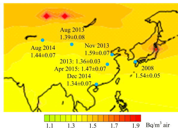
FIG. 7 Atmospheric ^{85}\text{Kr} concentration in China. The background is the annual surface ^{85}\text{Kr} concentration in 2006 [6]. The compare data in Japan is from Ref.[19]
