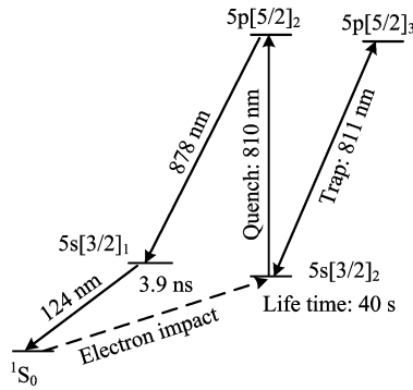
FIG. 1 Energy levels and transitions related to the ATTA measurement of Kr.
