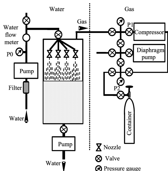
FIG. 4 Diagram of vacuum extraction system built at USTC.
