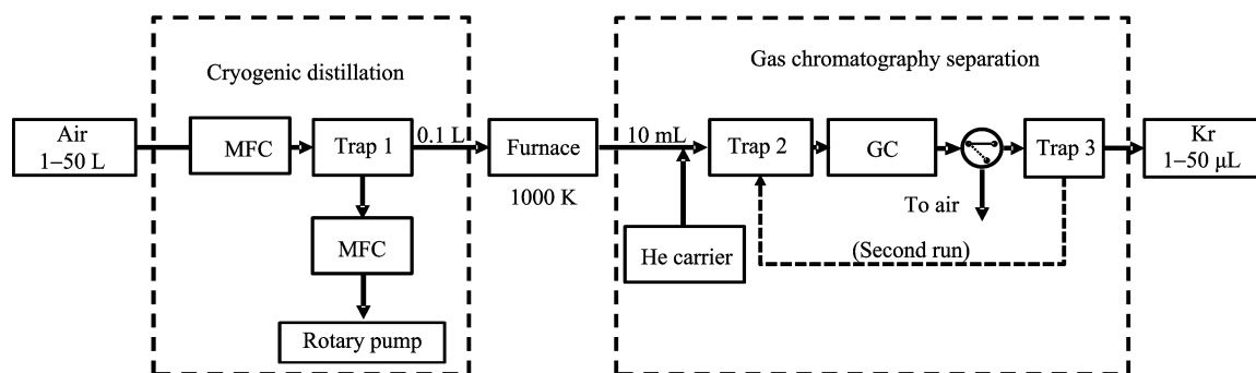
FIG. 5 Diagram of the krypton purification process. MFC: mass flow controller, GC: gas chromatography, trap: liquid-nitrogen cooled trap filled with activated charcoal.
