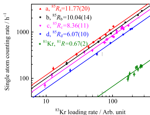
FIG. 3 Ratio between the ^{85}\text{Kr} counting rate and the ^{83}\text{Kr} loading rate measured by the ATTA-Hefei setup. Four commercial krypton gas samples were used, referred as samples a, b, c, and d. Samples a and c were produced in 2012 and 2007 respectively.
