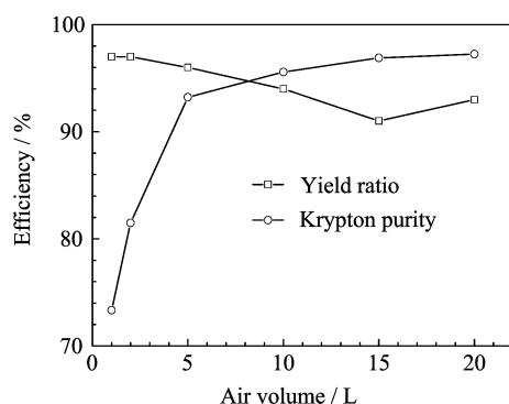
FIG. 6 Performances of the purification system at different ambient air size.
