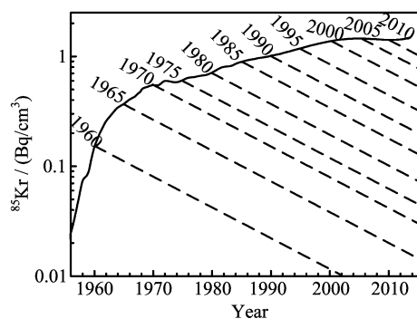
FIG. 8 Northern hemispheric ^{85}\text{Kr} activity as a function of time, extracted and combined from Refs.[31, 32]. Dashed diagonal lines represent radioactive decay since isolation from the atmosphere. Note that a logarithmic scale is used.
