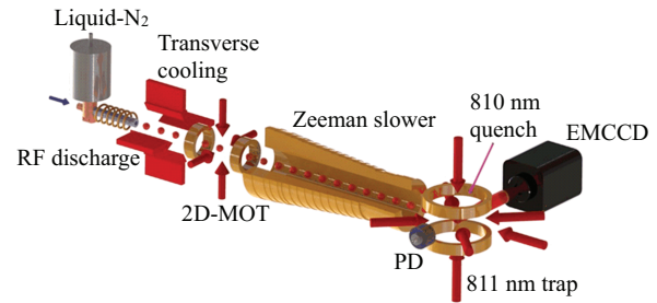
FIG. 2 Schematic of the ATTA instrument.
