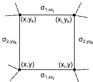
FIG. 5. A typical cycle in the Cartesian product graph.
