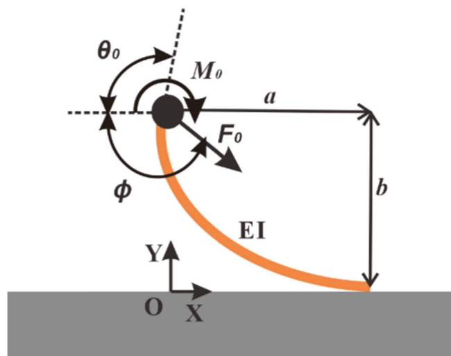
Figure 2. Diagram of large deflection cantilever's mechanical model.
