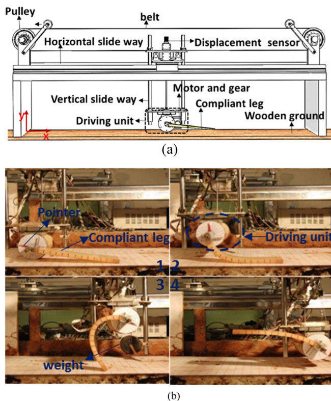
Figure 1. Single-leg locomotion platform. (a) Draft of the locomotion platform. (b) Snapshots of the compliant leg during one cycle in locomotion.
