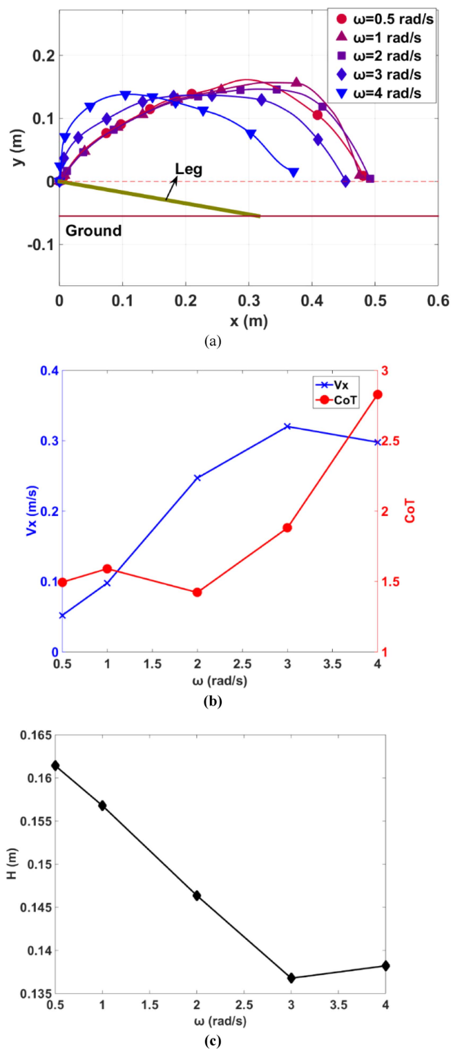
Figure 7. Simulation results of the single-leg locomotion platform.
