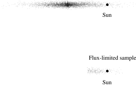
Figure 15: Small-number bias of the scale factor estimates derived from a synthetic population of sources where the true number of sources is known. Left panel: An edge-on view of a model Galactic source population. Right panel: The thick line shows N_G , the true number of objects in the model Galaxy, plotted against N_{\text{observed}} , the number detected by a flux-limited survey. The thin solid line shows N_{\text{est}} , the median sum of the scale factors, as a function of N_{\text{obs}} from a large number of Monte Carlo trials. Dashed lines show 25 and 75% percentiles of the N_{\text{est}} distribution.
