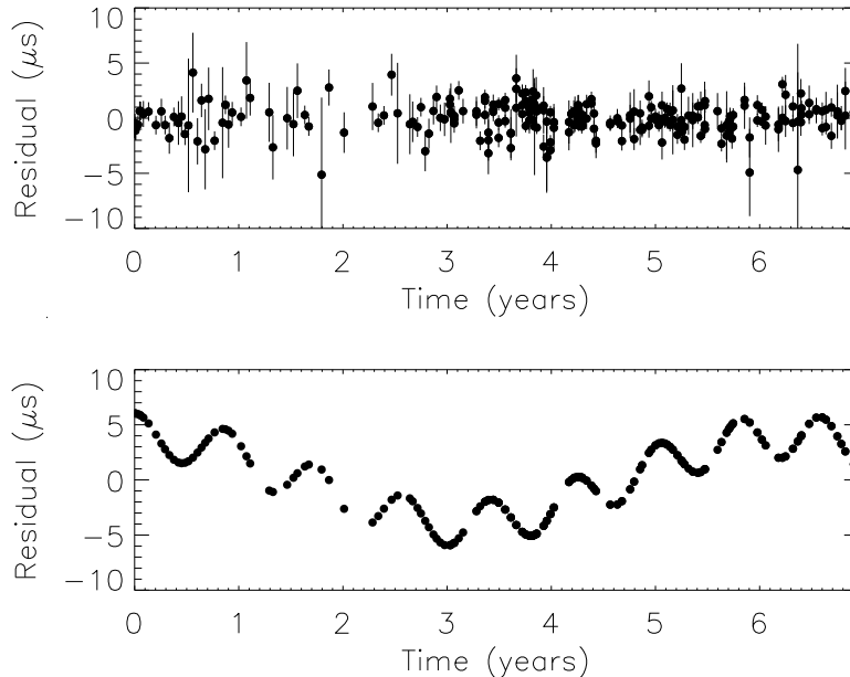
Figure 30: Top panel: Observed timing residuals for PSR B1855+09. Bottom panel: Simulated timing residuals induced from a putative black hole binary in 3C66B. Figure provided by Rick Jenet [161].
