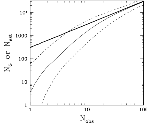
Figure 15: Small-number bias of the scale factor estimates derived from a synthetic population of sources where the true number of sources is known. Left panel: An edge-on view of a model Galactic source population. Right panel: The thick line shows N_G , the true number of objects in the model Galaxy, plotted against N_{\text{observed}} , the number detected by a flux-limited survey. The thin solid line shows N_{\text{est}} , the median sum of the scale factors, as a function of N_{\text{obs}} from a large number of Monte Carlo trials. Dashed lines show 25 and 75% percentiles of the N_{\text{est}} distribution.
