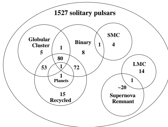
Figure 1: Venn diagram showing the numbers and locations of the various types of radio pulsars known as of September 2008. The large and small Magellanic clouds are denoted by LMC and SMC.
