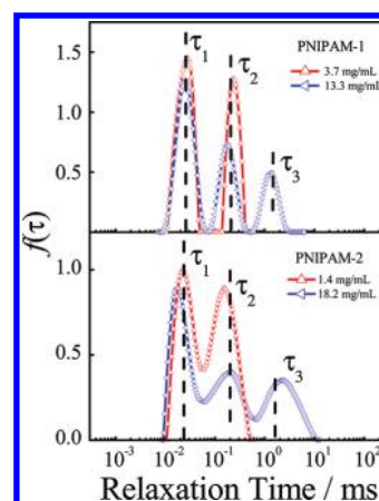
Figure 6. The relaxation time distribution for PNIPAM aqueous solution at different concentrations fit by CONTIN.
