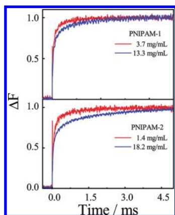
Figure 5. Time dependence of fluorescence intensity changes ( \Delta F ) from PNIPAM aqueous solution after the laser-induced temperature jump at different concentrations, where \Delta F is defined as [I_F(t) - I_F(0)]/[I_F(\max) - I_F(0)] .
