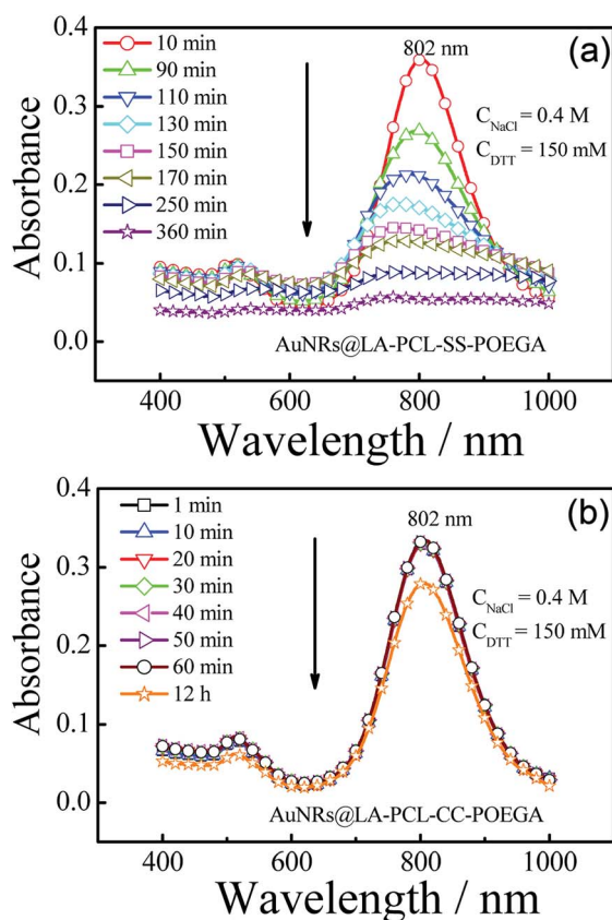
Fig. 4 Time-dependent absorption spectra of (a) AuNRs@LA-PCL-SS-POEGA and (b) AuNRs@LA-PCL-CC-POEGA aqueous solutions containing 150 mM DTT and 400 mM NaCl with an initial absorbance \approx 0.3\text{--}0.4 .
