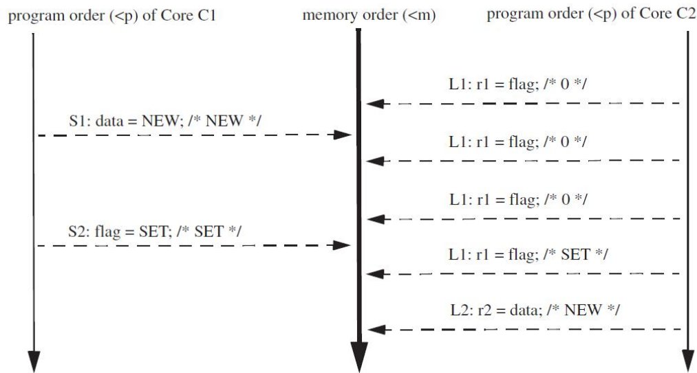
FIGURE 3.1: A Sequentially Consistent Execution of Table 3.1's Program.
