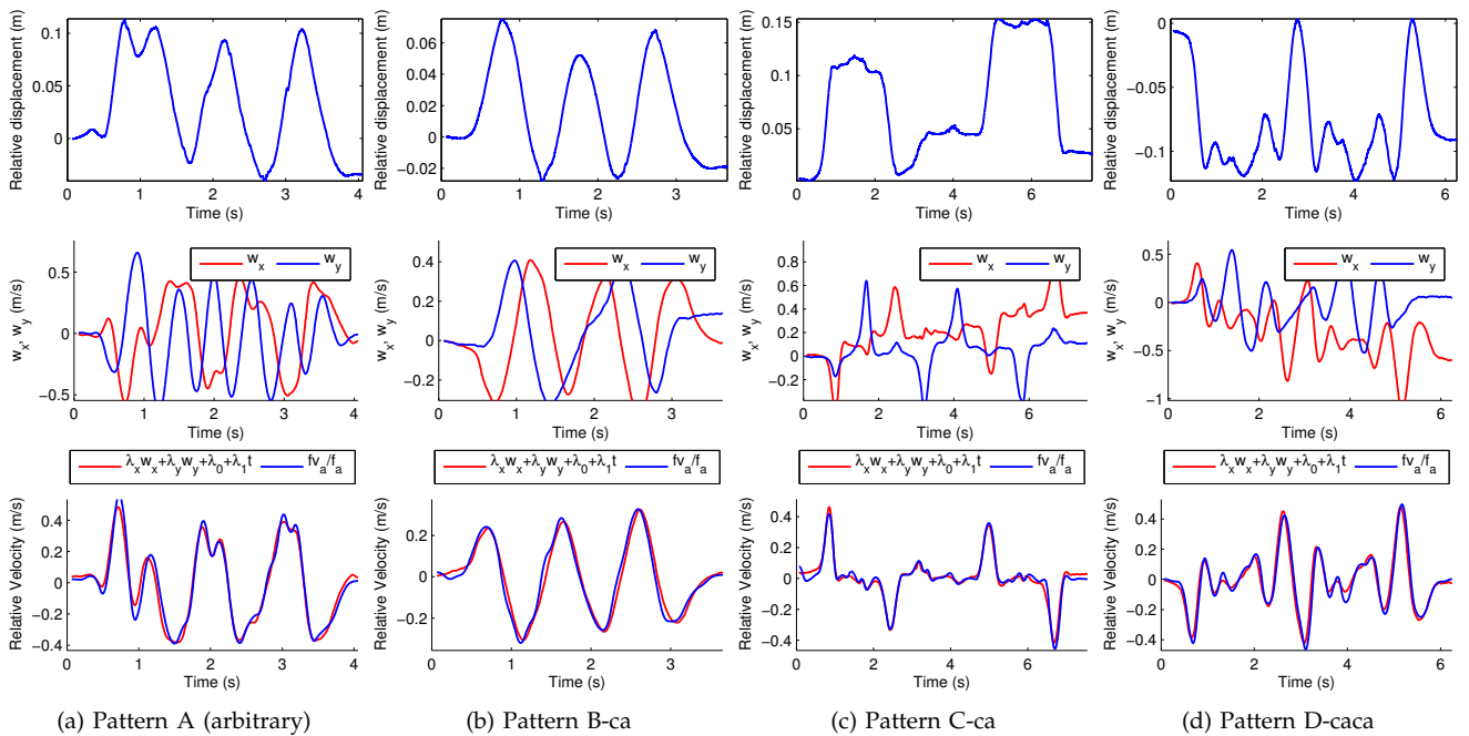
Fig. 7: Examples of direction finding which combines velocity from relative displacement \frac{v_a}{2\pi f_a} \phi(t) with the one from inertial sensors ( w_x(t) and w_y(t) ).
