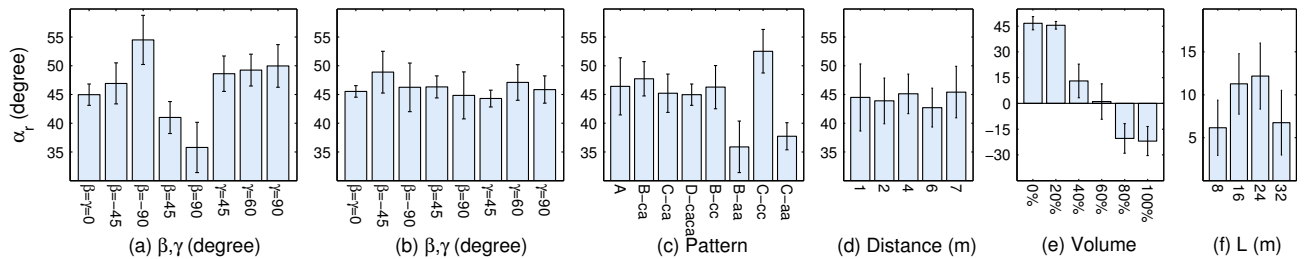
Fig. 4: Mean and standard deviation of \alpha_r (degree) affected by (a) \beta and \gamma when L = 8m (b) \beta and \gamma when L = 32m (c) motion pattern (d) non-line of sight (e) man-made multipath (f) multipath from the wall.
