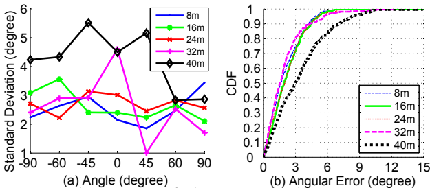
Fig. 5: The result of direction finding in an empty room when \beta = 0 and \gamma = 0 .
