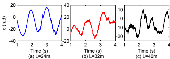
Fig. 6: The calculated phase \phi(t) .
