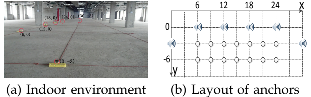
Fig. 11: Indoor localization testing prototype.
