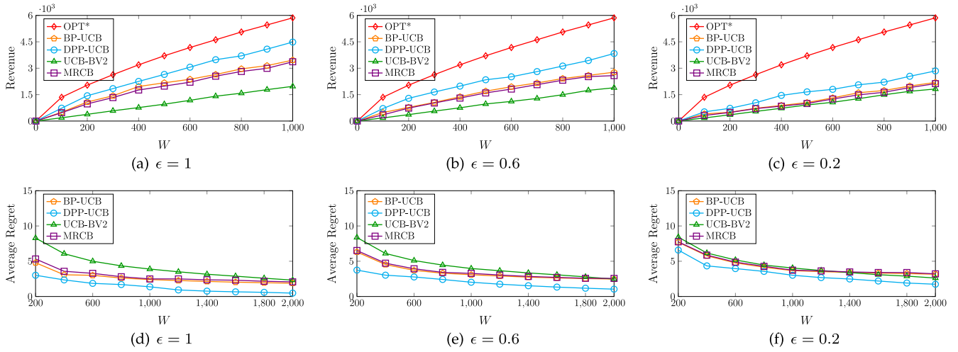
Fig. 5. Comparing the revenue/regret of the implemented online algorithms using the T-Drive dataset.
