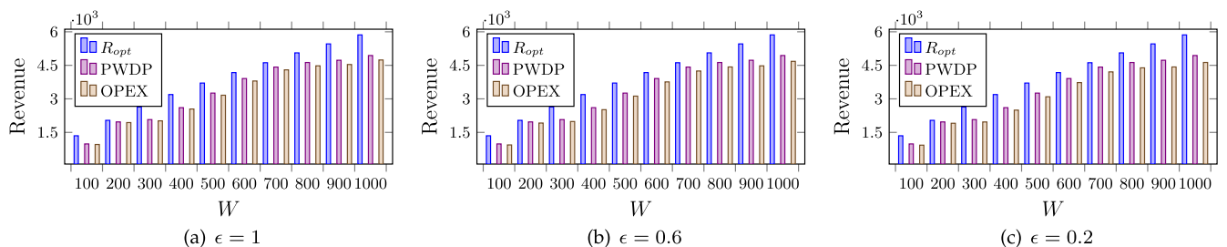
Fig. 4. Comparing the revenue of the implemented offline algorithms using the T-Drive dataset.
