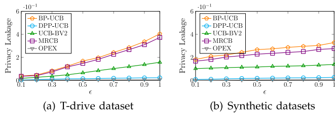
Fig. 8. Comparing the privacy leakage.
