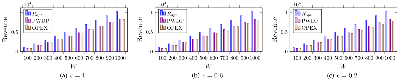
Fig. 6. Comparing the revenue of the implemented offline algorithms using the synthetic datasets.
