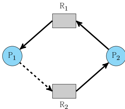
Figure: Unsafe State In Resource-Allocation Graph
