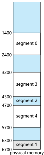
physical memory
