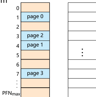
Physical memory
