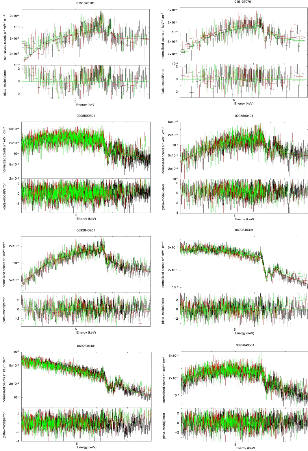
Fig. 2 The spectral fitting results for the eight XMM-Newton observations. The black , red and green points represent the data of PN instrument, MOS1 and MOS2 instruments, respectively.
