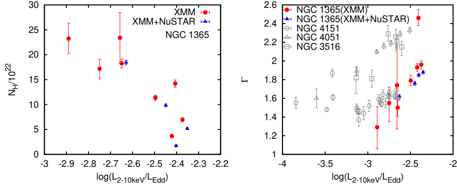
Fig. 3 Left panel: The correlation between N_H and \log(L_{2-10\text{keV}}/L_{\text{Edd}}) for NGC 1365. For comparison, we present the fitting results for XMM-Newton (red circles) and the joint analysis of XMM-Newton/NuSTAR (blue triangles). Right panel: The correlation of \Gamma - \log(L_{2-10\text{keV}}/L_{\text{Edd}}) , and we also present the correlation for other three variable AGNs.
