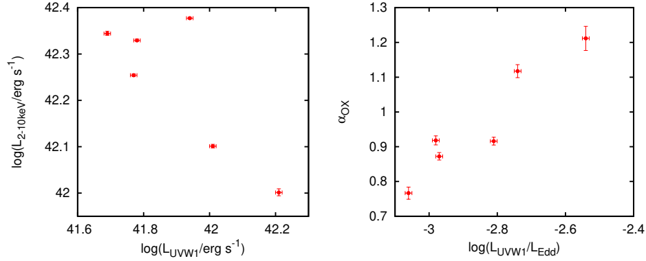
Fig. 4 The left panel and right panel represent the relations of L_{2-10\text{ keV}} - L_{\text{UVW1}} and \alpha_{\text{OX}} - \log(L_{\text{UVW1}}/L_{\text{Edd}}) , respectively.
