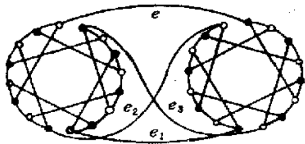
G_2
