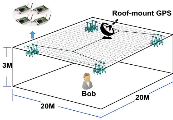
Fig. 9. The Secret-Focus prototype consists of 16 transmitter USRPs. The deployment area of our prototype is 20 \times 20 \times 3 m^3 .
