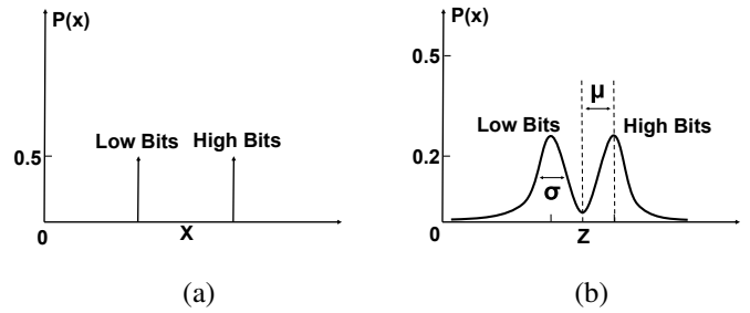
Fig. 3. (a) Alice generates low bits and high bits following amplitude based modulation. (b) shows a typical distribution of bits received by Bob. Received bits follow a mixed (complex) Gaussian distribution.
