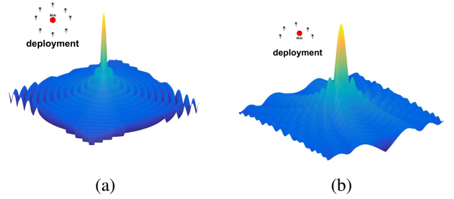
Fig. 6. (a) Simulation results of RSS distribution in a 1m by 1m area around Bob. It is clear that the energy is sharply focused around the target location. In (b), we decrease the number of transmitters to 30, and place them on a half circle. Note the target receiver is also not placed at the center. As can be seen, even though the energy focus is wider, the peak is still very pronounced compared to other locations.
