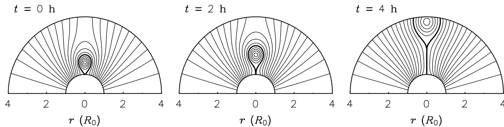
Fig. 2. Magnetic configurations at three separate times, showing an eruption of the flux rope right after the catastrophic point (after Sun and Hu, 2005).
