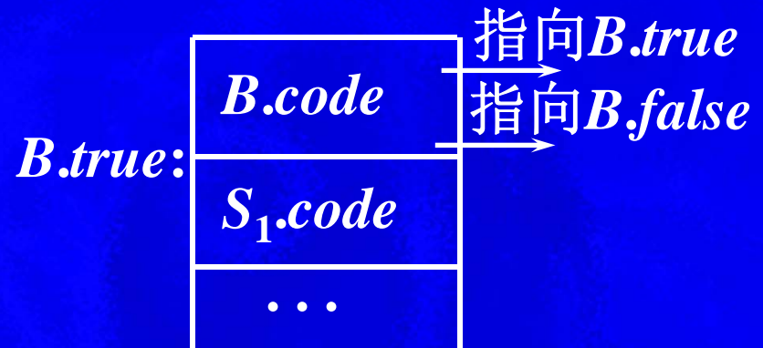
(a) if-then
