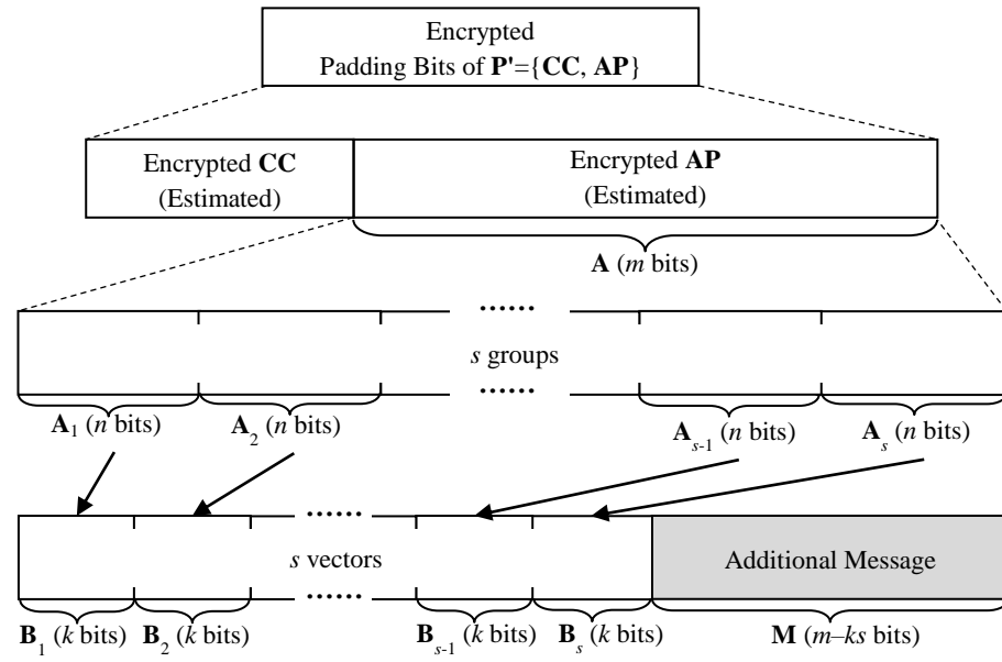
Fig. 8 Procedure of data embedding
