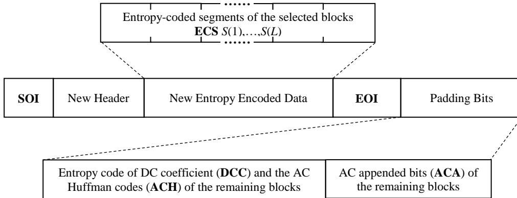
Fig. 5 Syntax of the new JPEG bitstream
