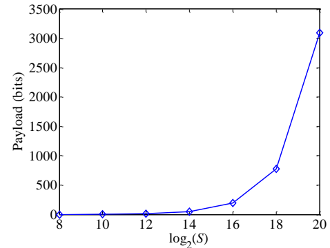
Fig. 15 Payload vs. image resolution
