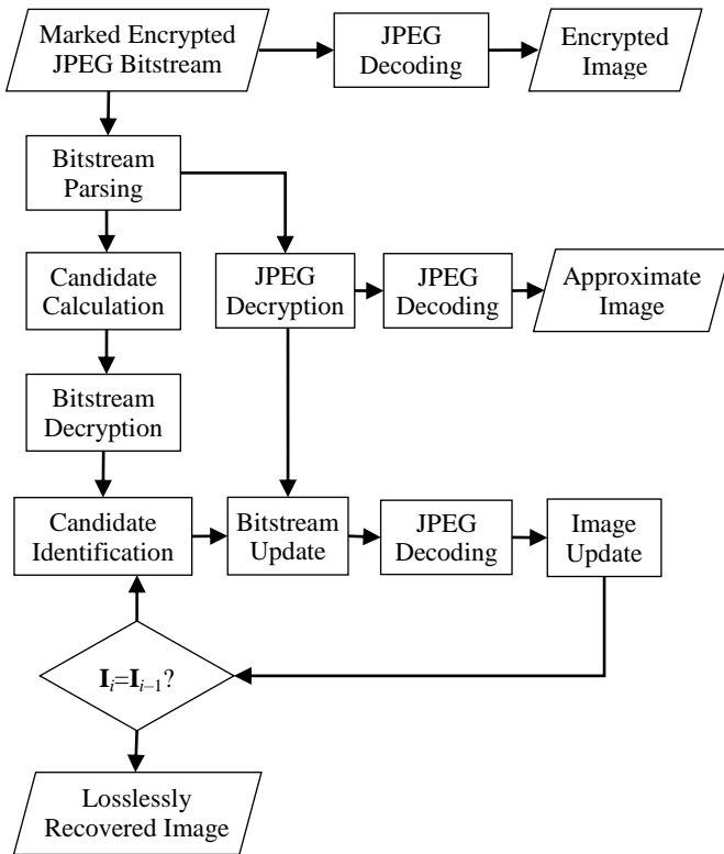
Fig. 9 Flow chart of iterative recovery
