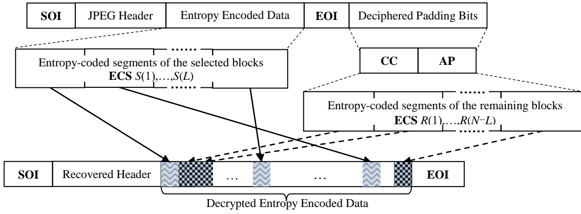
Fig. 7 Procedure of JPEG decryption
