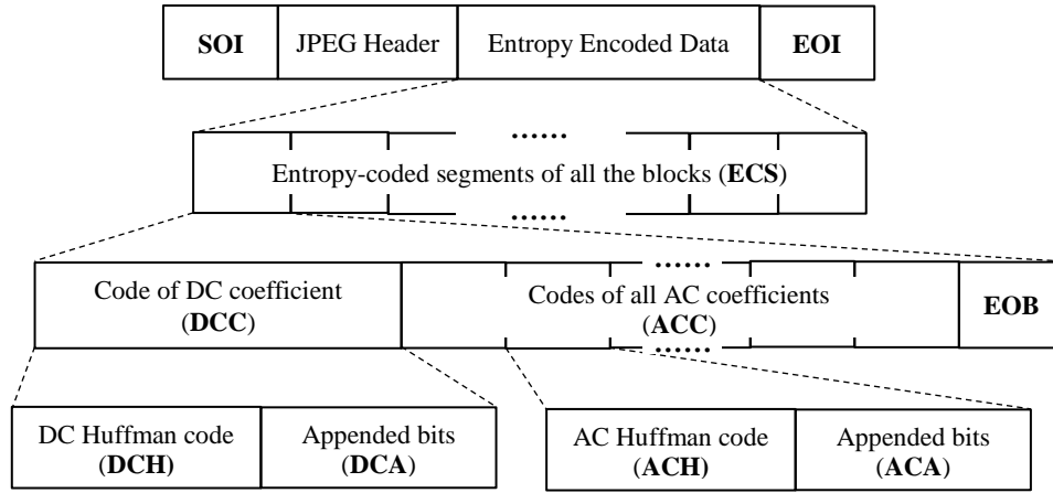
Fig. 4 Simplified syntax of JPEG baseline. SOI , EOI and EOB stand for start-of-image, end-of-image and end-of-block respectively. Acronyms in the parentheses are used in the discussion for brevity.
