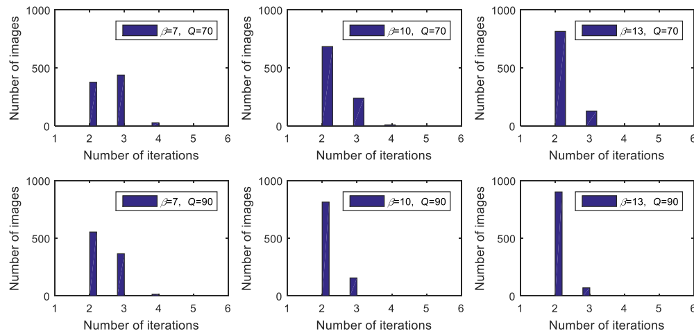
Fig. 14 Convergence of iterative recovery
