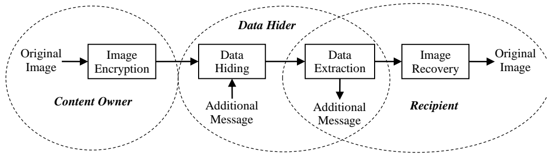
Fig. 2 General framework of RDH-EI
