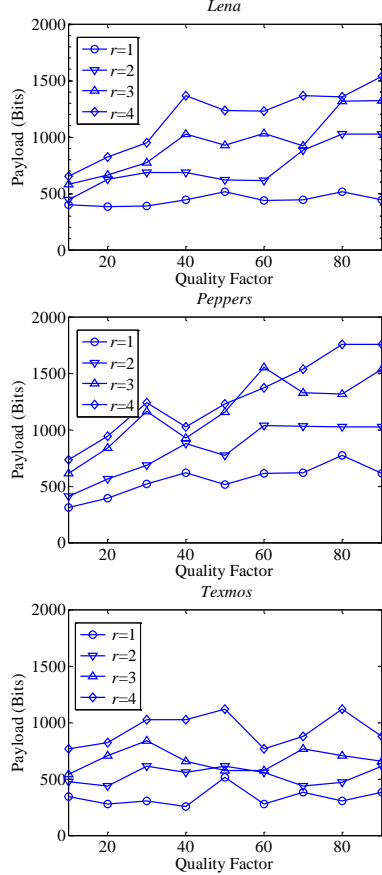
Fig. 13. Payload vs. quality factor
