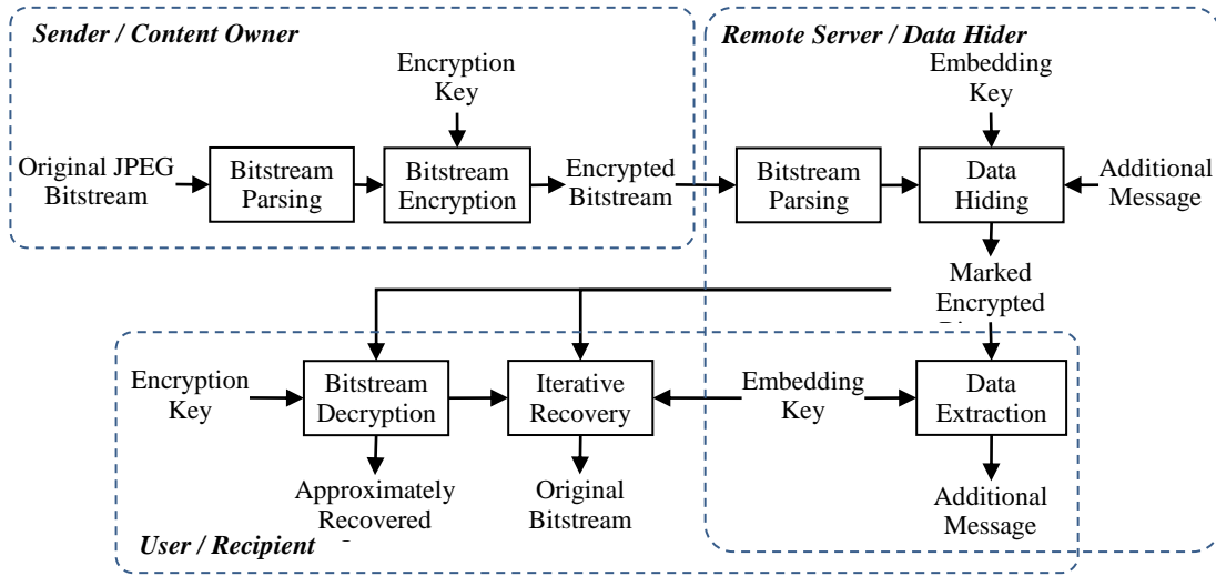
Fig. 3 Framework of the proposed method
