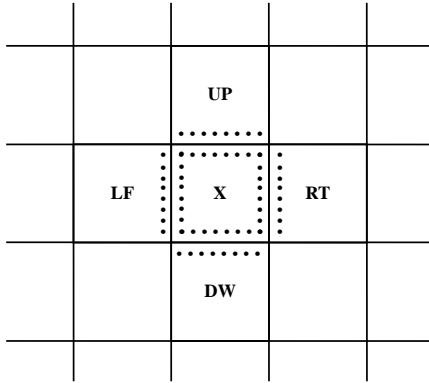
Fig. 10 Blocking artifacts
