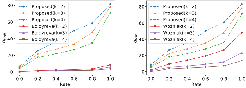
Fig. 2. The security of proposed method ( p = 0.80 ) and Boldyreva, Wozniak.
