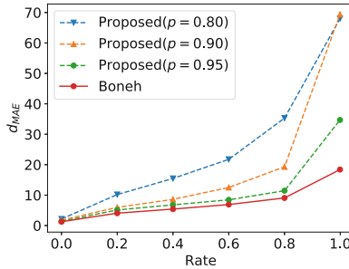
Fig. 3. The security of proposed method and Boneh.
